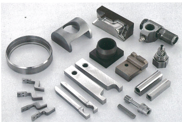
Spare Parts Transport Grippers
